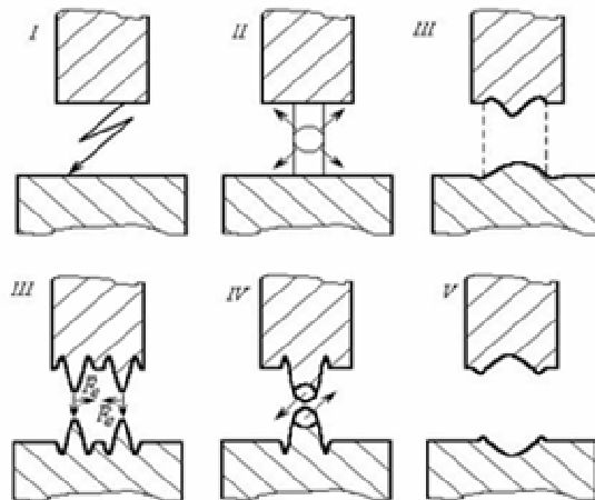
Fig 4 The model of electro erosion process proposed
