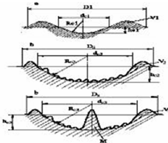
Fig.1 Types of craters obtain during the dimensional processing by electro erosion ( D_1 , D_2 , D_3 ) – crater diameters together with the wave; d_{c1} , d_{c2} , d_{c3} – diameters of three crater types; h_{c1} , h_{c2} , h_{c3} –crater depth; M – meniscus; V – val.[8].
