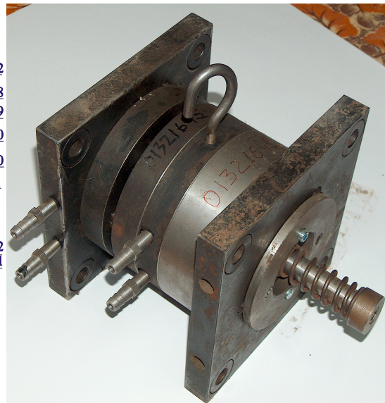
Figure 1. Mold of plastic gear wheels in the precessional gear.
