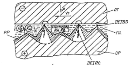
Fig.1. The fundamental scheme of processing through complex erosion
