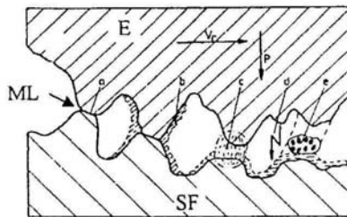
Fig.2. The elementary working area
