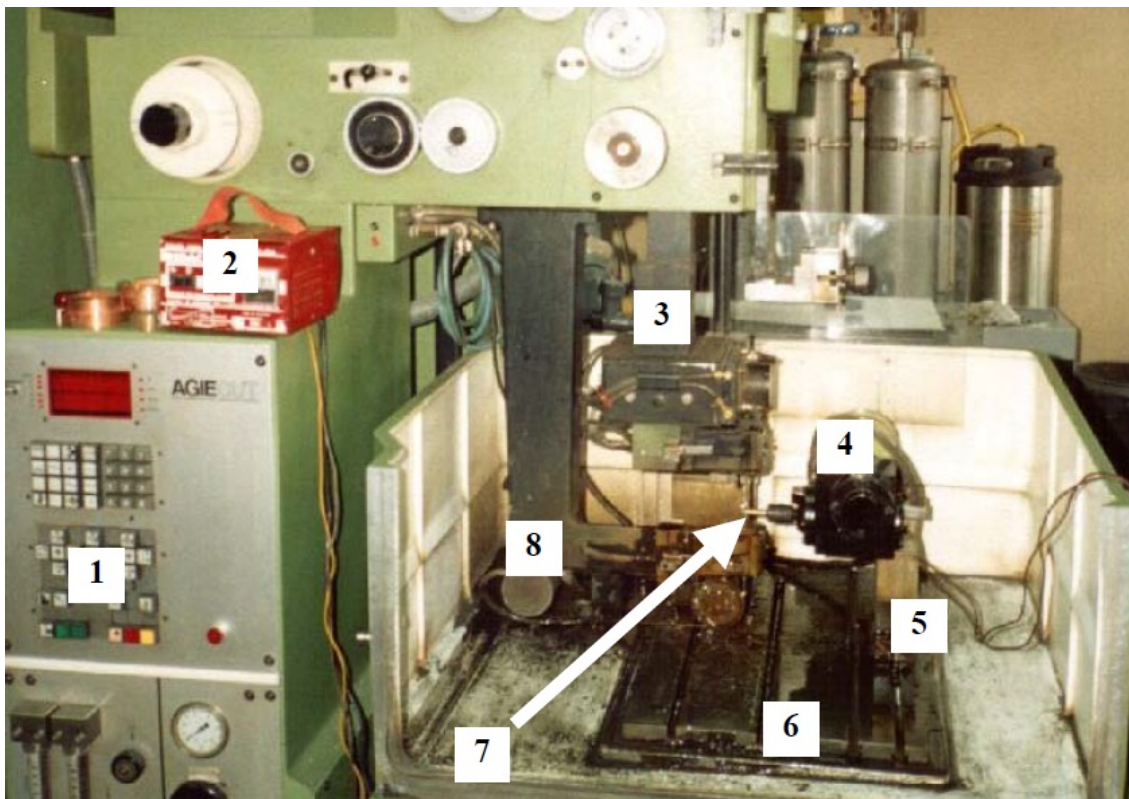
Figure 3. Experimental stand
