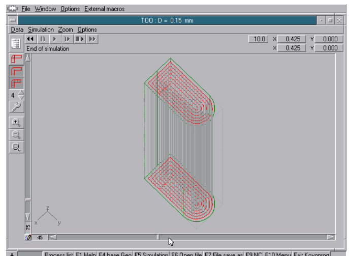
Figure 6. The wire electrode's trajectory
