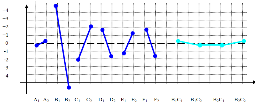
Figure 9. Effects exerted upon the size of the S/N ratio regarding the dimensional precision
