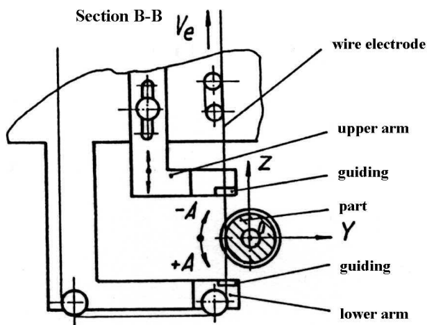
Figure 1. The device used in processing revolution surfaces
