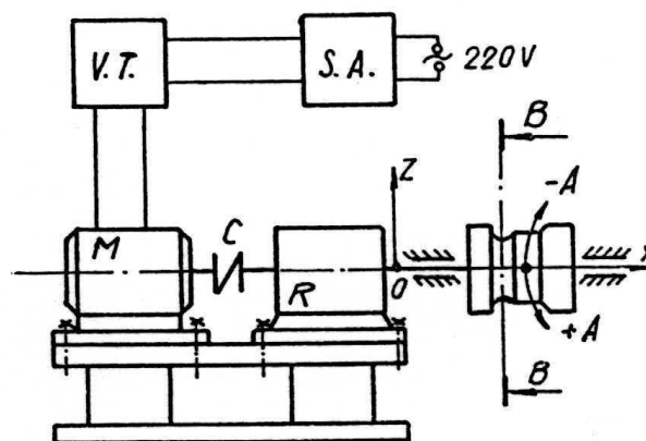
Figure 1. The device used in processing revolution surfaces
