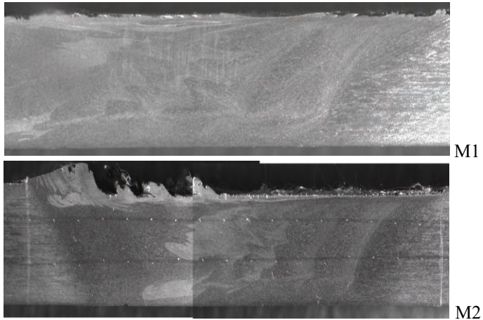
Figure 3. Macroscopic analysis of processed material samples The microscopic analysis for M1 and M2 samples, performed with the microscope in Figure 1g (according to SR EN ISO 17639:2022 and SR EN
