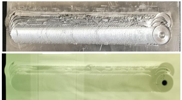
Figure 2. Top surface appearance and Rx image - SFSP processed material - EN AW 6082 (5mm)
