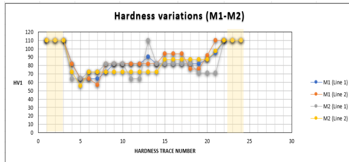
Figure 5. Graphs of hardness variation of processed materials
