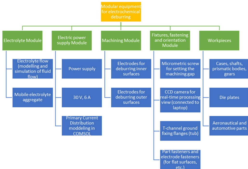
Figure 8. Equipment's modules
