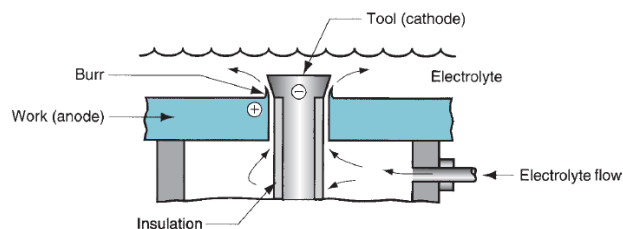
Figure 2. Basic phenomenology [2]
