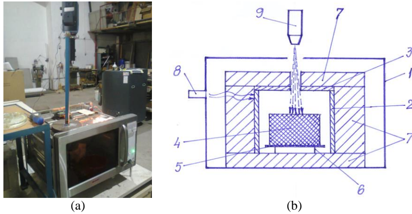
Figure 1. Experimental microwave device
